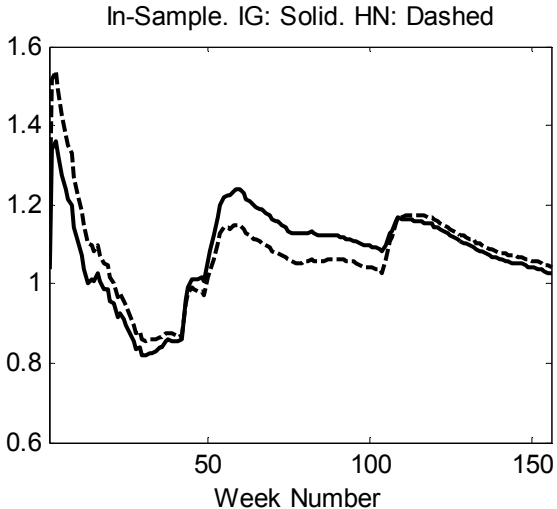
Figure 7: Cumulative RMSE across weeks. Heston-Nandi and Inverse Gaussian GARCH models Deep in-the-money call options only
